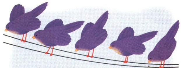
6. birds
