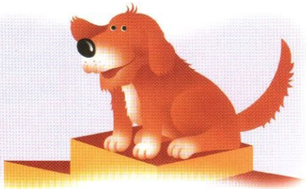
1. dog
